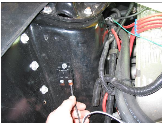
Figure 7-3 R.H. Shock Tower
