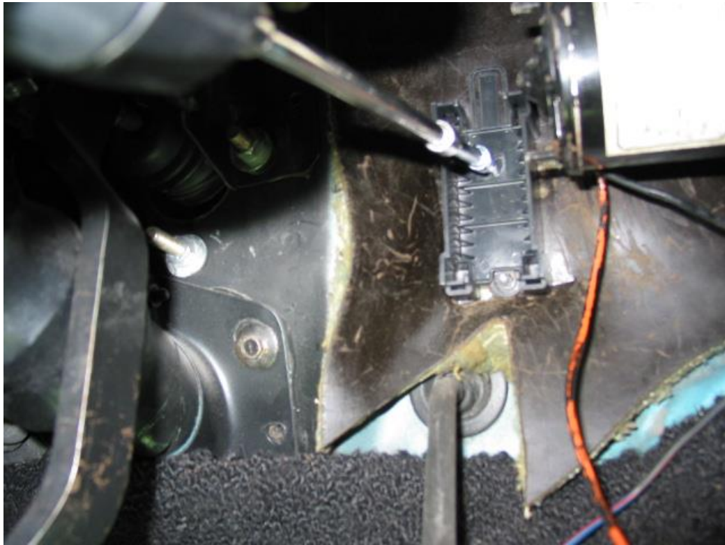
Figure 6-1 Fuse Block Base Position
