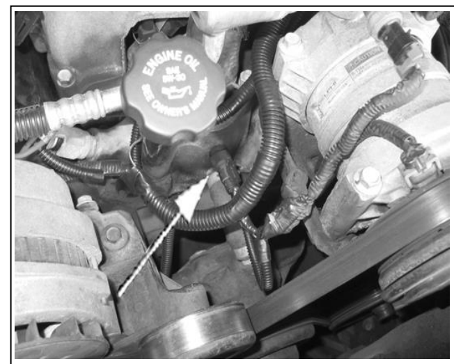
FIGURE 6.16 ECT Sensor
