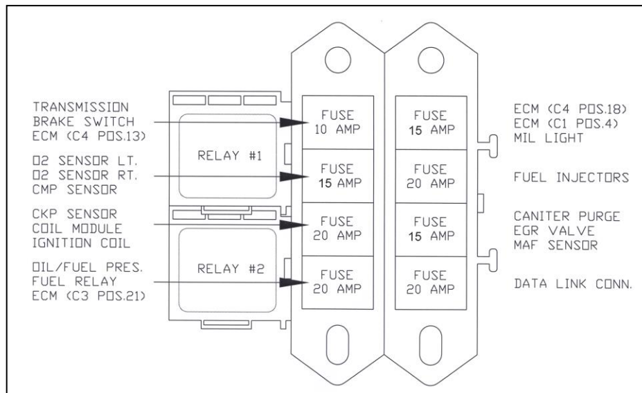
FIGURE 6.20 Fuse Identification
