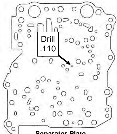
Separator Plate
