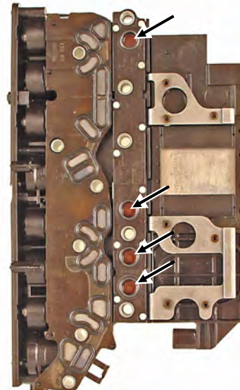
Gen 1 TEHCM Pressure Switch Locations
