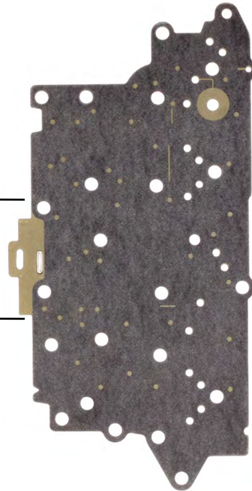
Front Steel Cover Plate (Rear Side) w/Bonded Gasket
