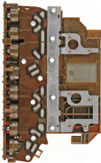
Gen 2 TEHCM No Pressure switches
