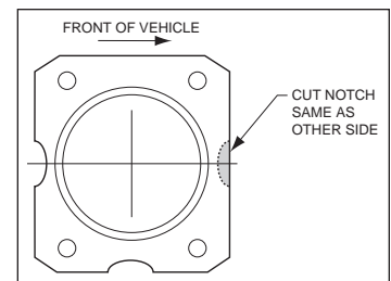
Figure 4. Flange Modifications
