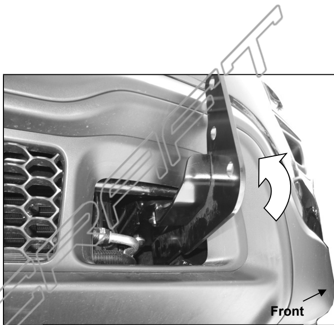
(Fig 11B) Rotate the Bracket to meet the mounting holes for the tow hooks
