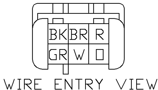
Figure 6. UEGO Connector Pinout
