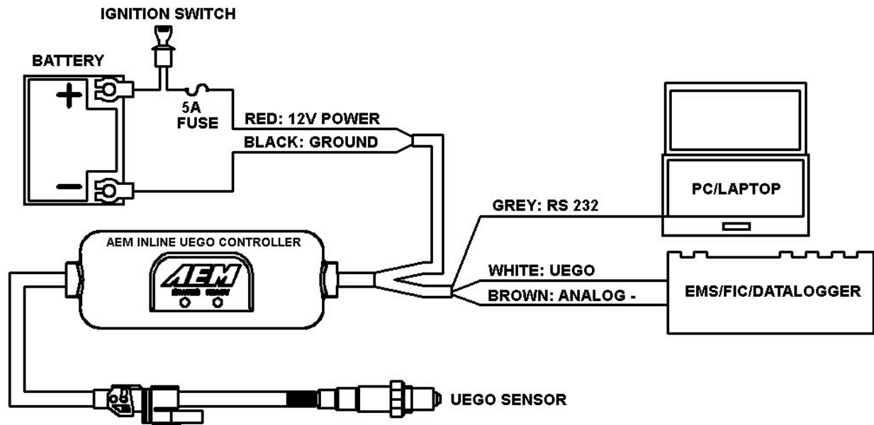
Figure 1. Wiring Schematic
