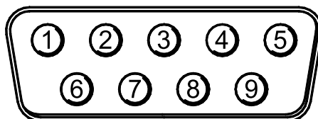
Figure 5. Wire View of RS-232 (DB-9) Male Plug
