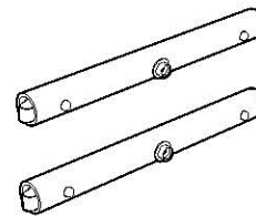
Bow Coupler #1 & #4 Bows Part #573.77 Qty. 2
