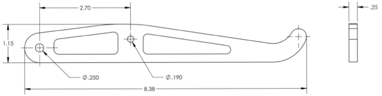
Dimensions in Inches
