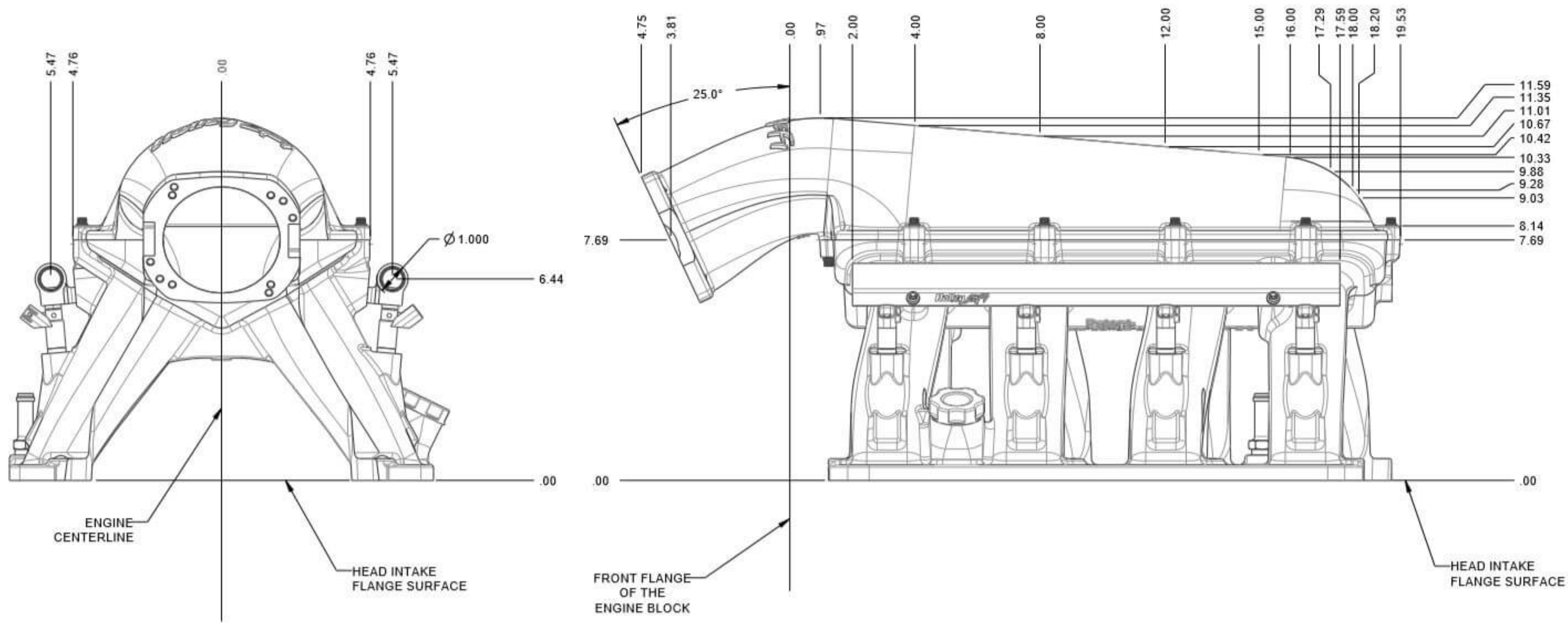
HI-RAM INTAKE MANIFOLD WITH EFI PLENUM TOP - OUTLINE DIMENSIONS
