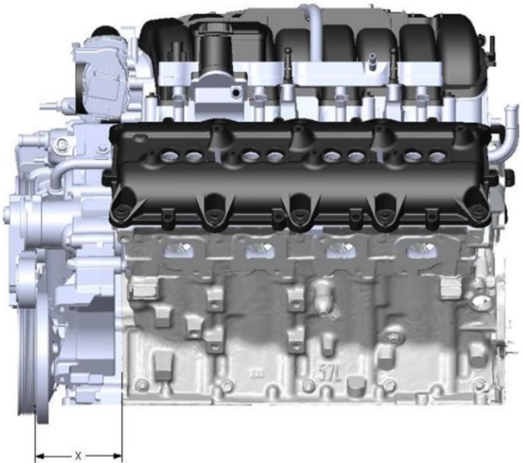
Figure 1-Belt Alignment
