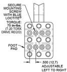
FOOT PAD DETAIL
