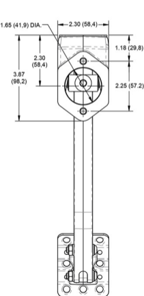
FOOT PAD DETAIL
