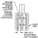
FOOT PAD DETAIL
