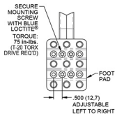
FOOT PAD DETAIL
