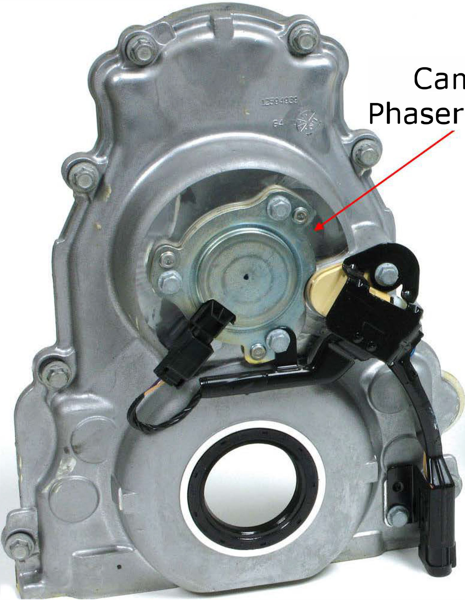
VVT Timing Cover
