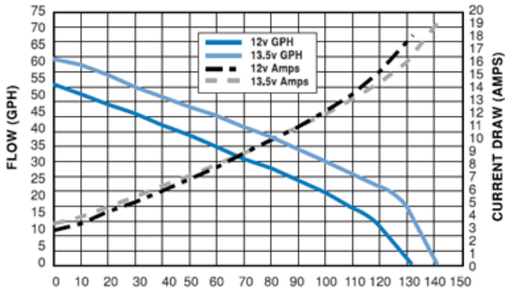
Flow vs. Pressure @ 12 and 13.5 VDC in Stoddard Solvent
