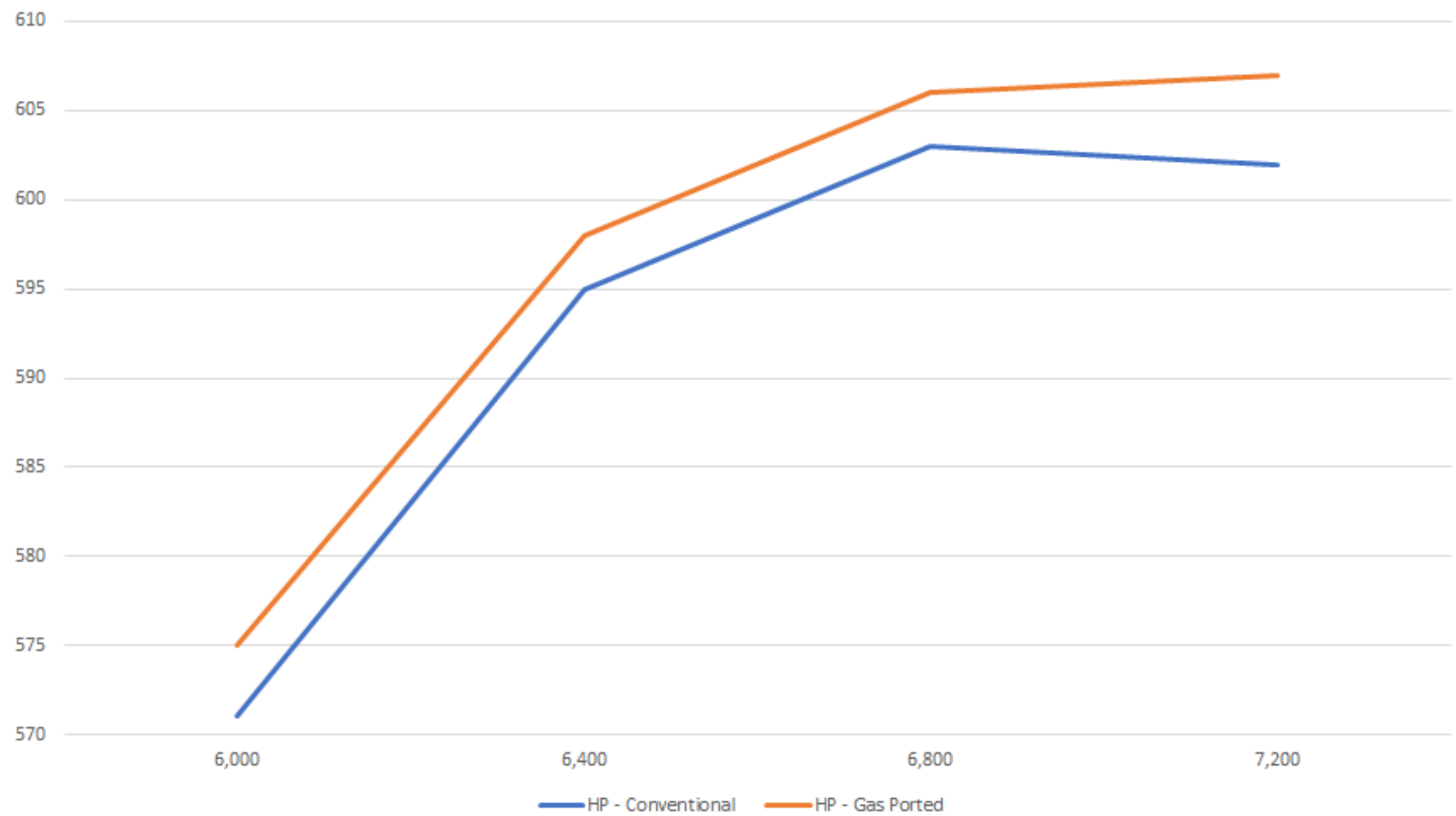
Horsepower Comparison
