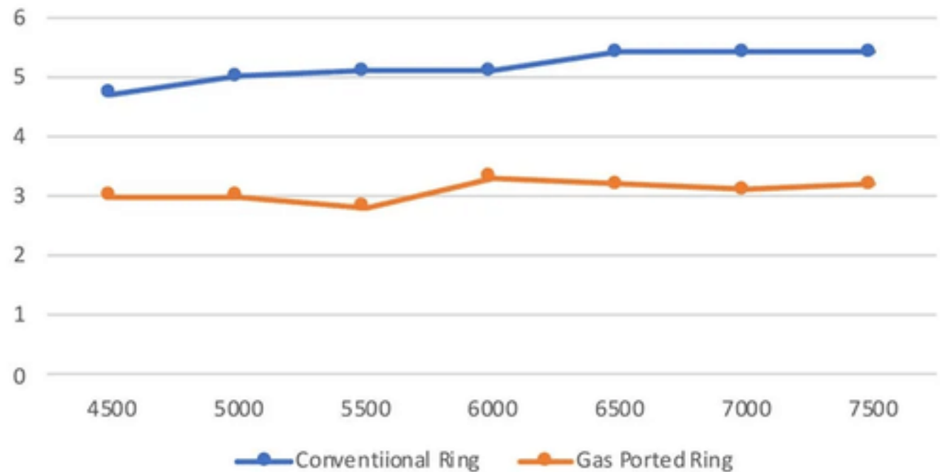
LS Engine Blow-By Comparison (cfm)
