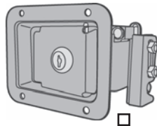
Rotary Latch Paddle Handle, Right, Qty - 1, Left, Qty - 1, Part Number 446.76 and 446.77
