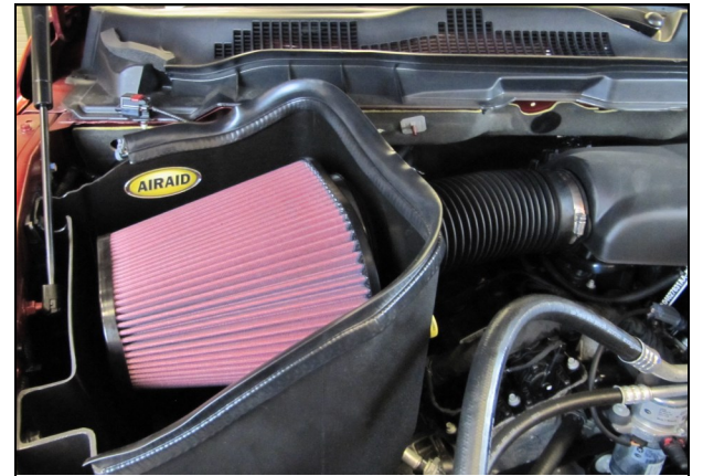
12. Install the Airaid Premium Filter onto the Filter Adapter inside the Cool Air Box. Install the Weatherstrip onto the Cool Air Box as shown, with the contour rolling away from the Filter.
