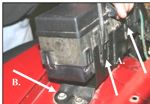
8. A.) On the right fender, pry two tabs away from the fuse box, lift it up and set it off to the side. B.) Next, remove and save the outside bolt from the fuse box mount. It will be re-used in step #14.
