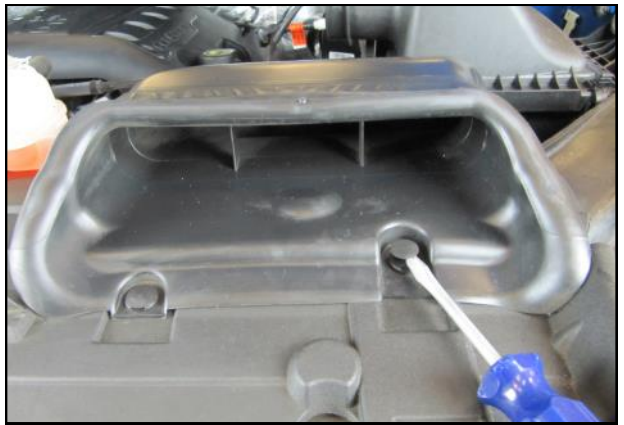
4. Using a standard blade screwdriver, gently pry up the center posts of the plastic rivets in the air inlet and remove them.
