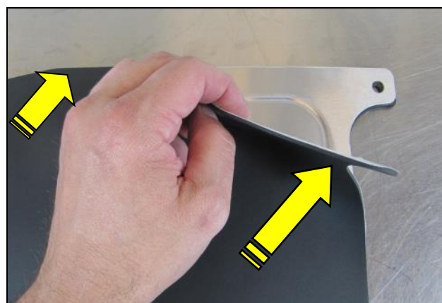
19. Remove the protective film from the top of the Air Box Lid. Prepare the underside for the Lid Gasket by cleaning it using a prep-sol or equivalent. Carefully apply the self adhesive Gasket onto the Lid as shown.
