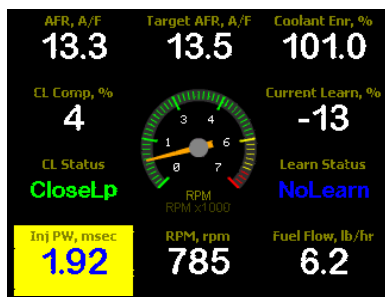
AIR/FUEL RATIO Multi-Gauge Engine below 160° F (NoLearn)
