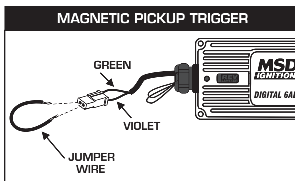
Figure 10 Checking for Spark with the Mag Pickup.
