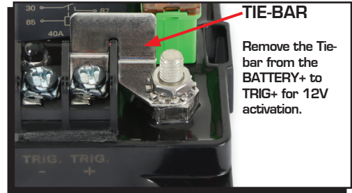
Figure 5 1 Channel Tie-bar removal for Ground activation
