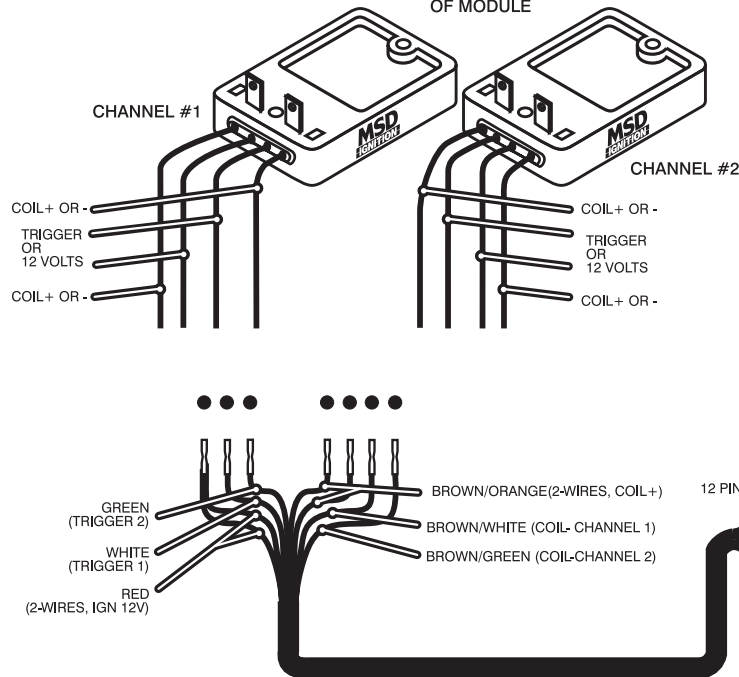
Figure 7 Your Wiring.
