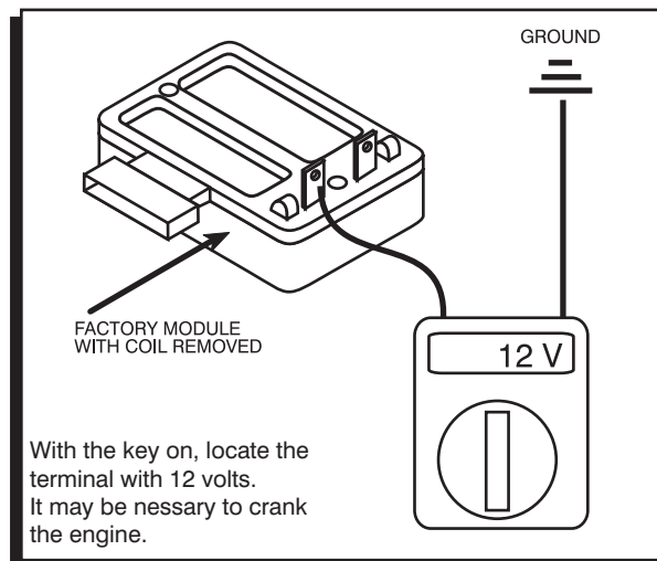
Figure 2 Identifying 12 Volts.
