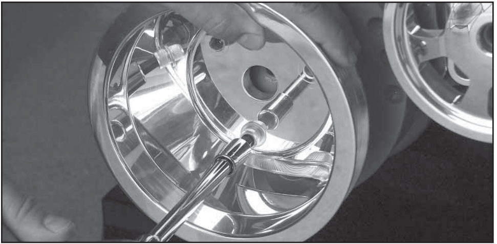
Figure 12: Install Crankshaft Pulley
