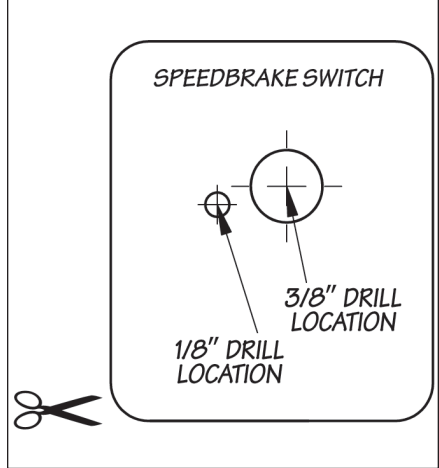
Figure 22- Use only when drilling from the rear
