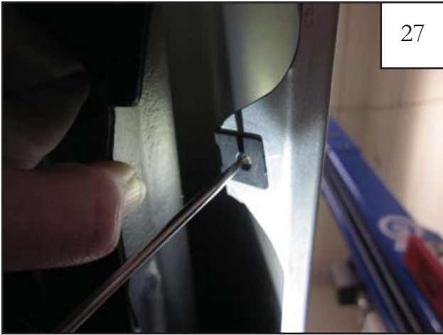
Using awl to poke hole through Tab using Clip installed in Step 26 as a guide. With Clip installed, tuck liner back in. Two locations
