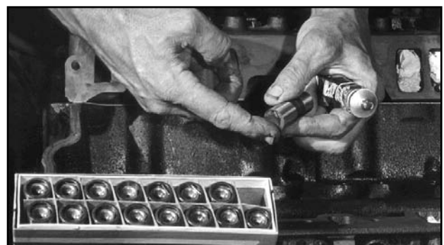
Figure 8. Apply a generous amount of assembly lube to each lifter bottom.
