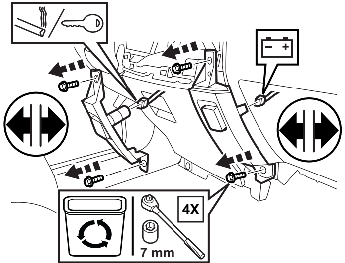
29 AUTOMATIC WITHOUT CENTER CONSOLE
