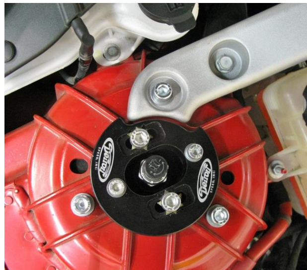
Figure 10 - Install Strut Assembly
