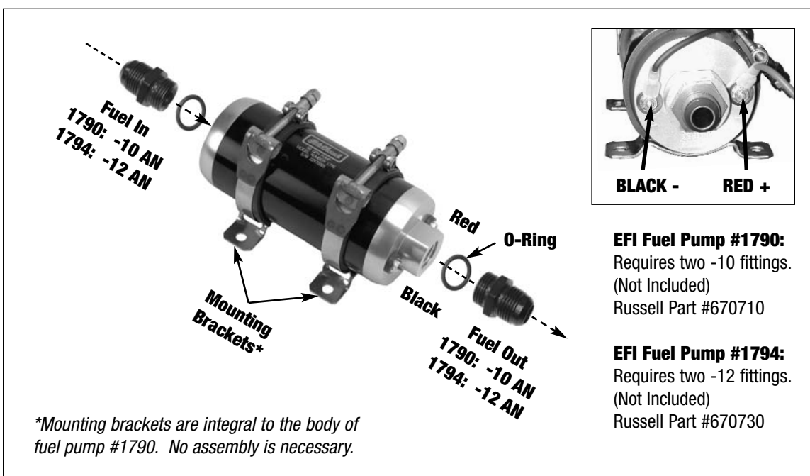
Figure 2 - Fuel Pump Fitting Assembly (1790 Shown)
