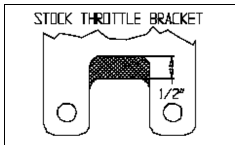
Figure 2 Remove material in the shaded area on stock throttle brackets to clear the intake manifold.
