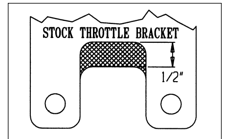
Figure 1 - Stock Throttle Bracket Remove material in shaded area on stock throttle brackets to clear the manifold.
