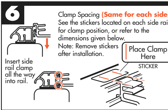
SHORTBED (3 clamps)
