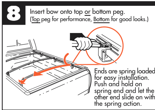
SHORTBED (3 clamps)
