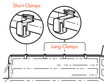
LONGBED (4 clamps)
