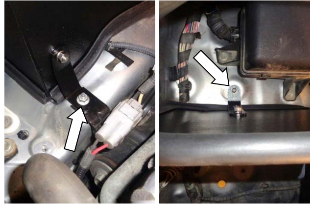
22. Fasten bracket (23) to vehicle with previously removed stock harness bracket nut. Fasten bracket (3) with M6 screw (6), lock washer (5), and flat washer (4). Tighten fasteners between airbox and brackets (23) and (26).
