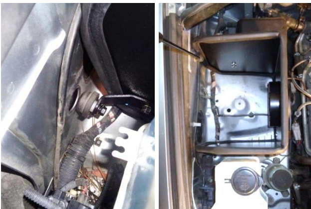
21. Set assembled airbox in vehicle, inserting the rubber bushing into its hole in the fender. If necessary, adjust alignment of brackets (23) and (26).
