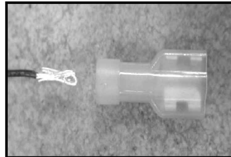
When crimping the temp. probe wires, strip back the insulation, then fold wire back on itself to double thickness
