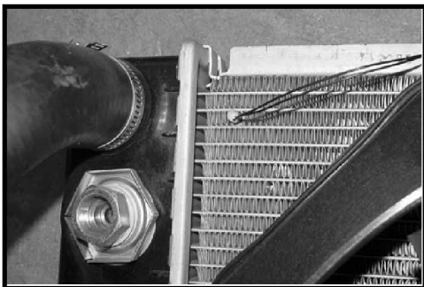
Install the temp. probe near the inlet hose, leaving 1/4" of the probe protruding from the core.
