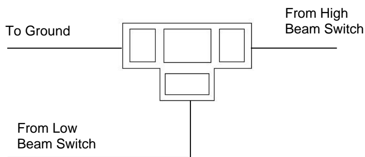
3-Wire Pigtail
