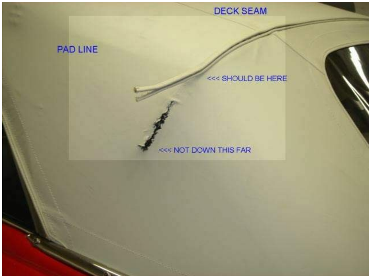
Fig. 13-42 — Tacking Outboard of Seams
