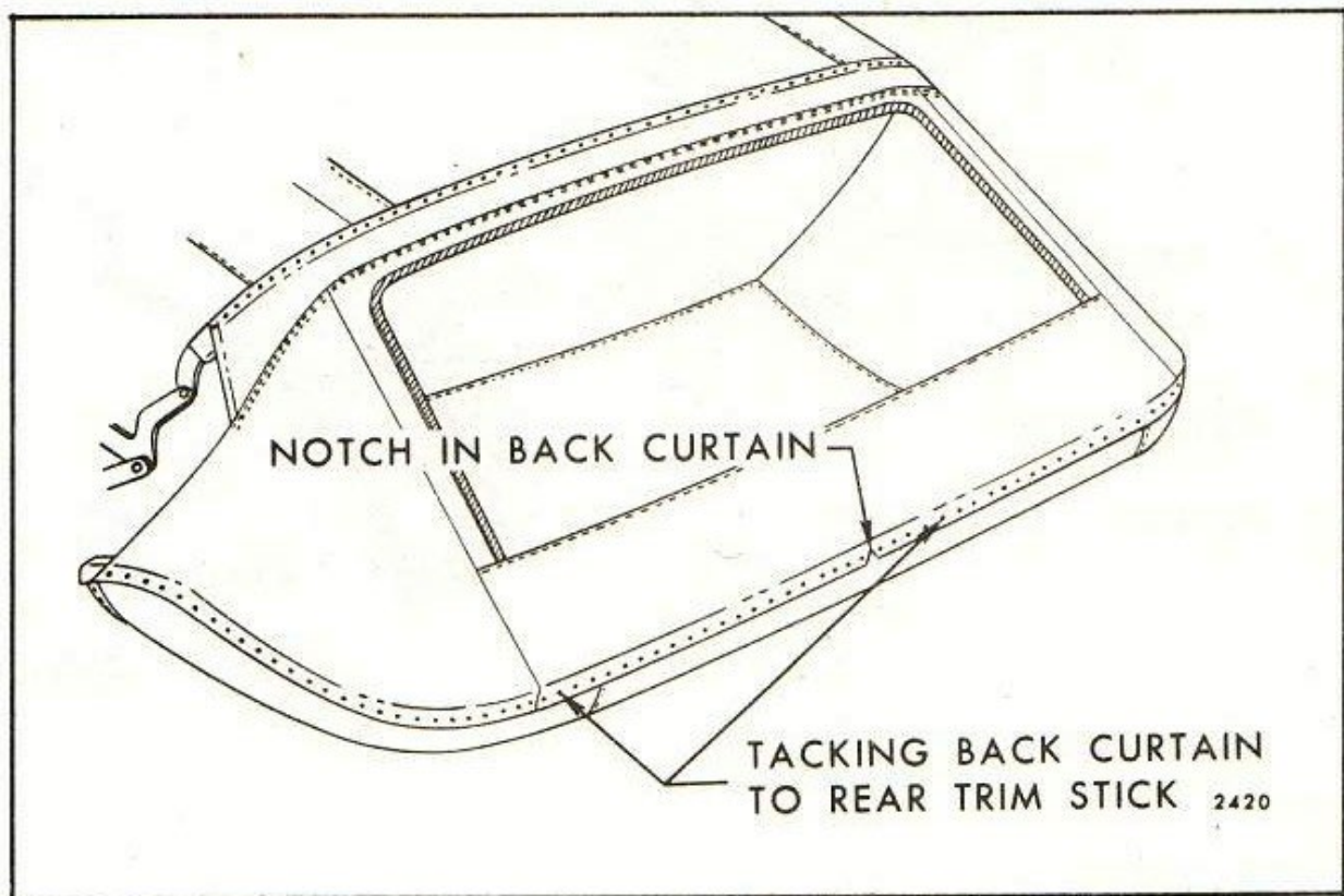
Fig. 13-17 — Back Curtain Installation
