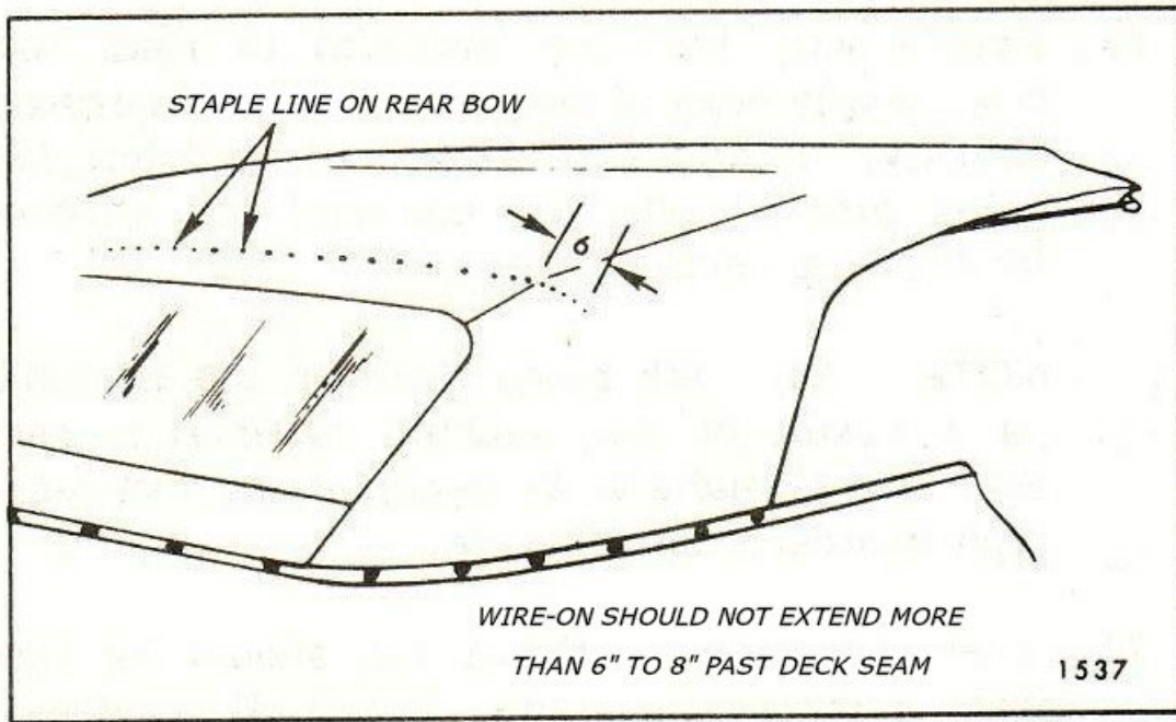
Fig. 13-42 — Tacking Outboard of Seams
