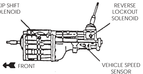
BORG-WARNER (T56) 6-SPEED MANUAL TRANSMISSION
