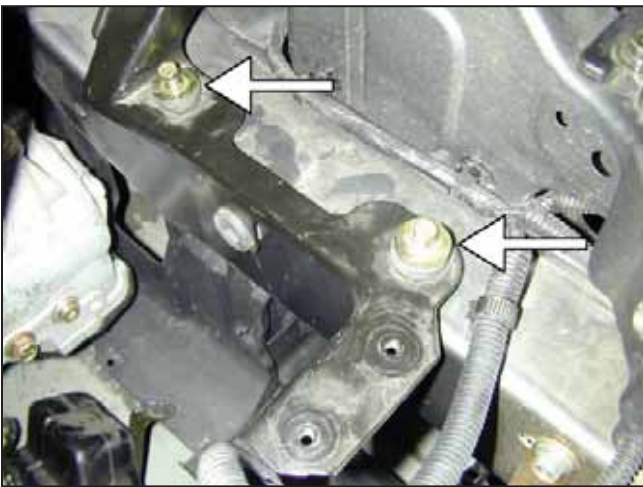
g. Remove lower mounting bracket.
