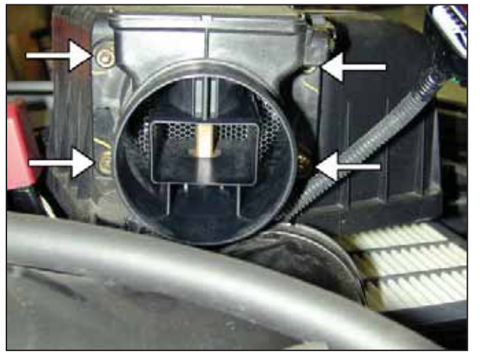
d. Loosen the four nuts that hold the MAF sensor to the airbox. Carefully set aside the MAF sensor.
