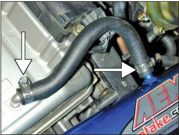
f. Install the supplied breather hose as shown. Secure both ends with supplied 3/4" hose clamps.
