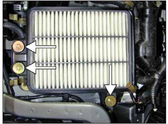
f. Loosen the three bolts holding down the air box. Remove air box and snorkel from vehicle.
