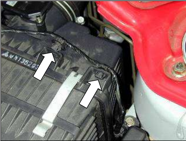
e. Unclip the Mass Air Flow (MAF) sensor wiring harness from the air filter housing.
