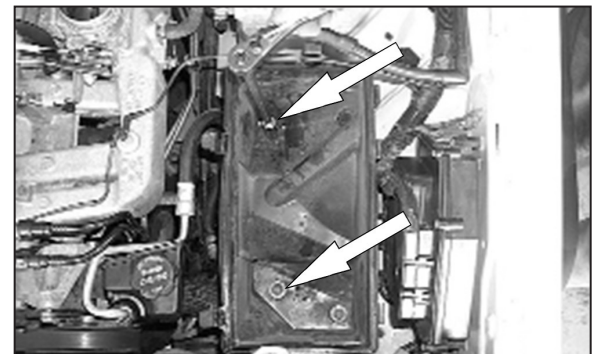
6. Loosen and remove the two bolts that secure the lower air cleaner assembly, then remove lower airbox from vehicle. NOTE: K&N Engineering, Inc., recommends that customers do not discard factory air intake
