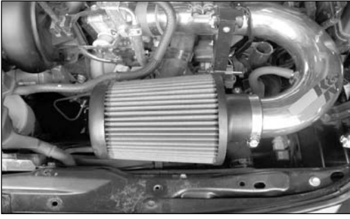
42. Install the K&N Filtercharger onto the intake tube and secure with the provided hose clamp as shown.
