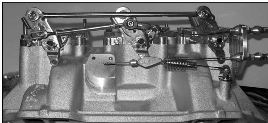
Photo 7 - Completed Installation
