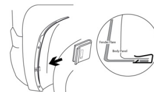
U-Clip
