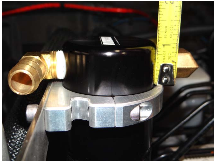
Step 19: Set height between 1" and 1" 1/8 as shown and tighten clamp.
