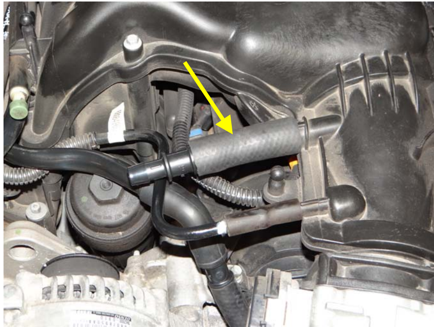
Step 8: Insert other end of 3" 5/8 hose to intake nipple.
