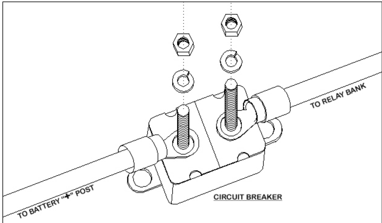
Figure 3: Circuit Breaker
